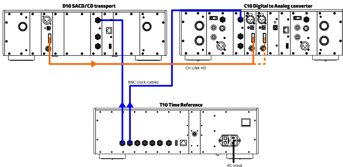
D10 SACD/CD transport - C10 - T10 connection when CLOCK_SYNC equipped
