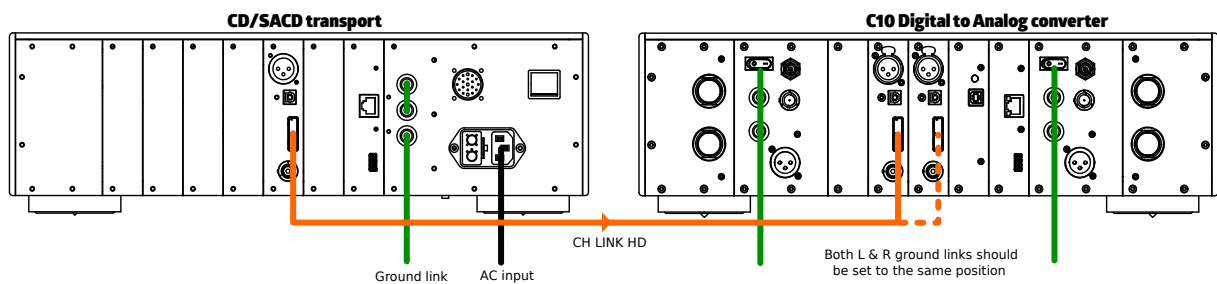
Simple CD/SACD transport - DAC connection
