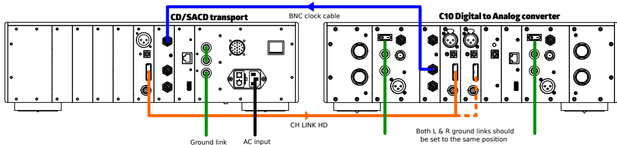
CD/SACD transport - DAC connection with CLOCK_SYNC
